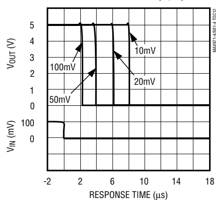
RESPONSE TIME FOR VARIOUS INPUT OVERDRIVES (V OHL )
