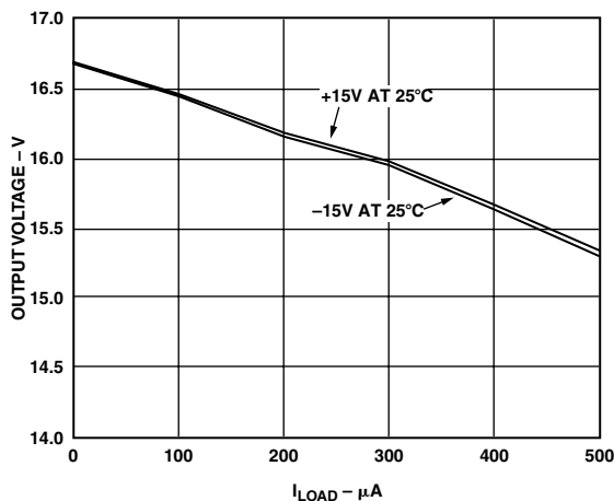
Figure 5. +15\text{ V}/-15\text{ V} Output Voltage vs. Load Current, Current Boost Configuration
