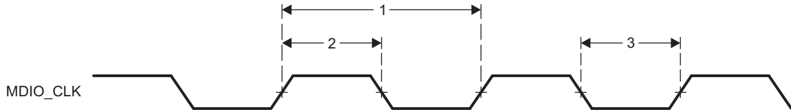
Figure 7-4. MDIO_CLK Timing
