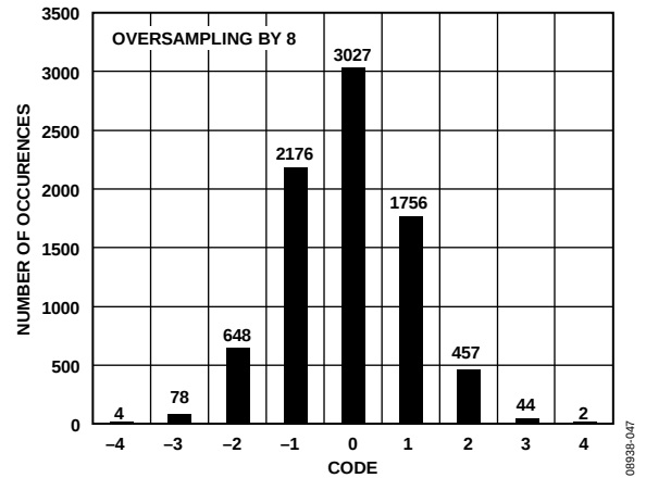
Figure 49. Histogram of Codes—OS \times 8 (9 Codes)
