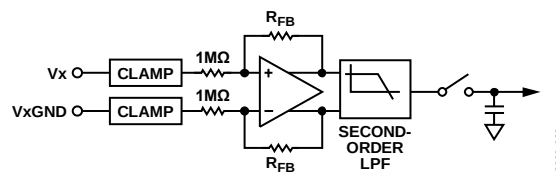
Figure 31. Analog Input Circuitry
