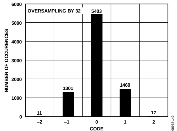
Figure 51. Histogram of Codes—OS \times 32 (5 Codes)
