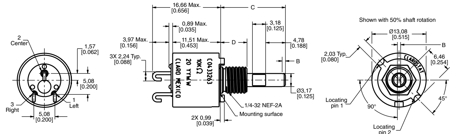
Dimensional Drawing (For reference only: mm [in].)
