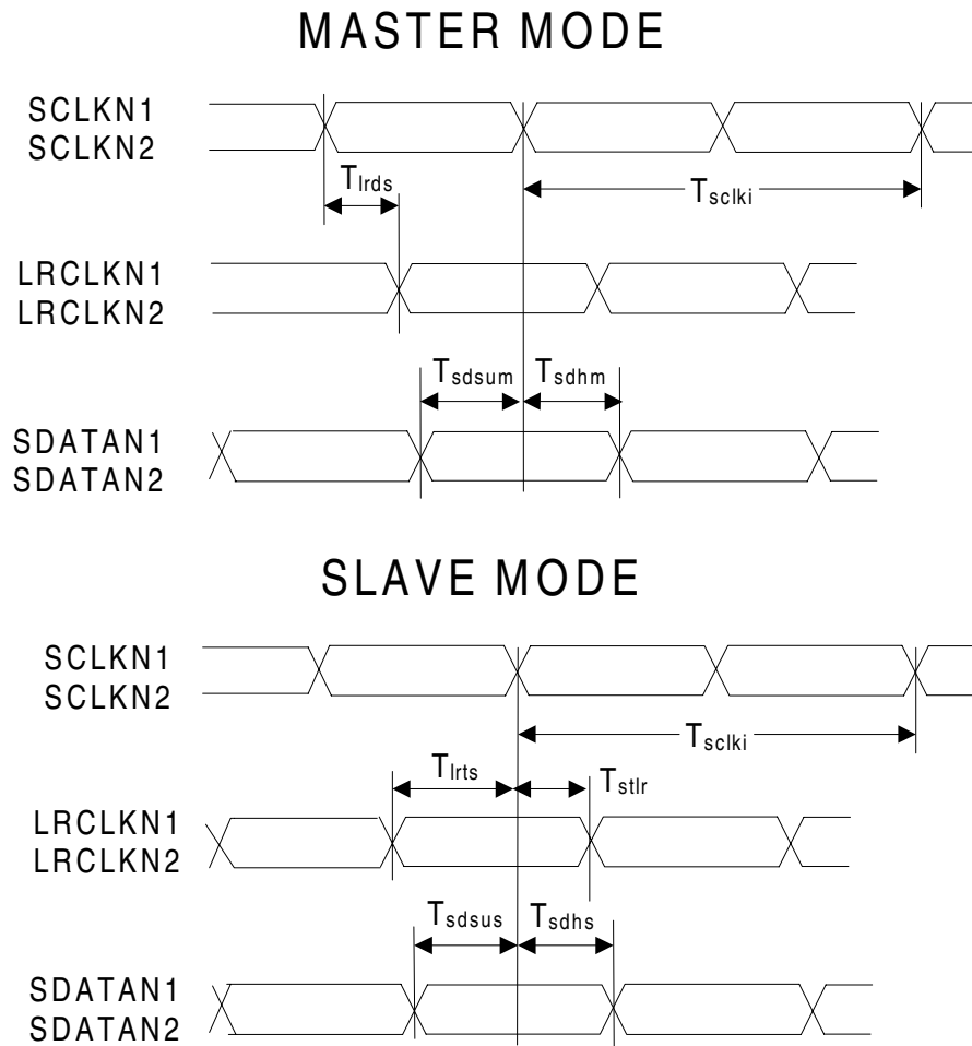
Figure 9. Digital Audio Input Data, Master and Slave Clock Timing
