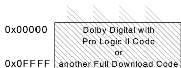
Figure 40. Non-Paged Memory
