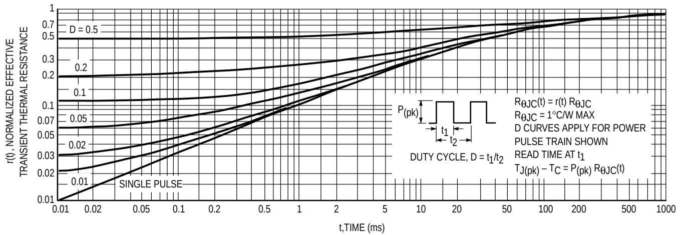
Figure 13. Thermal Response
