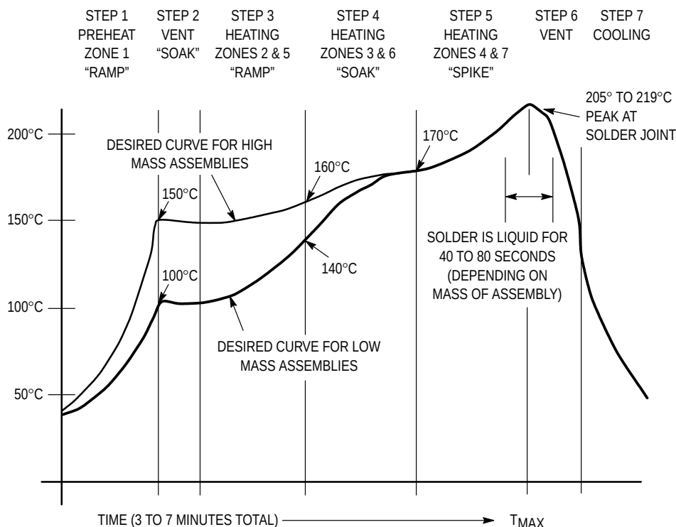
Figure 18. Typical Solder Heating Profile for D 2 PAK
