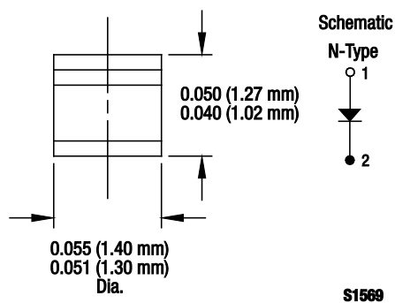
Figure 5. -203 Package
