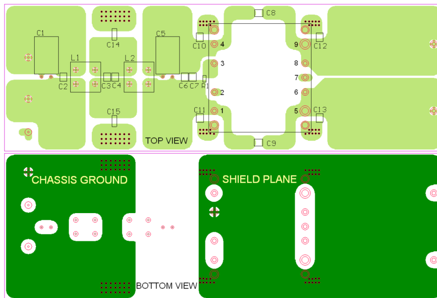
Recommended Layout With Input Filter
