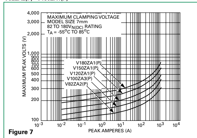
V82ZA2(P) - V180ZA1(P)
