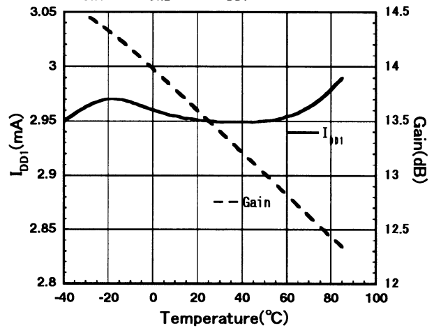
I_{DD1} , Gain vs Temperature
