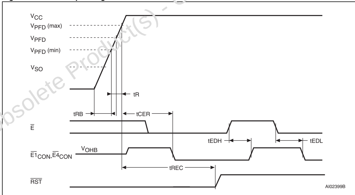
Figure 10. Power-up timing
