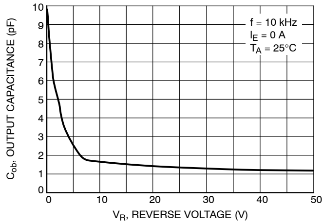
Figure 9. Output Capacitance
