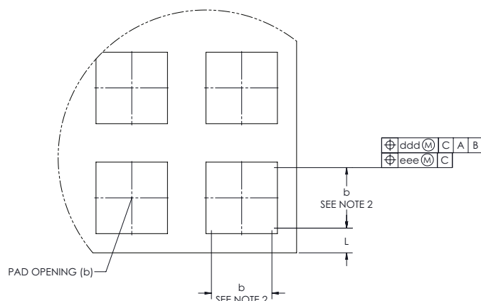
DETAIL A (SECTION VIEW)
