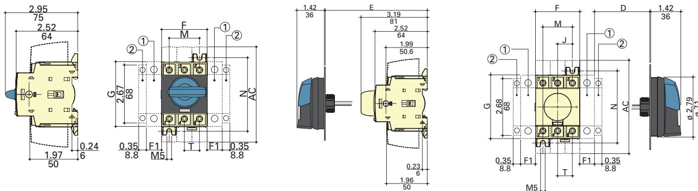
Direct handle operation
