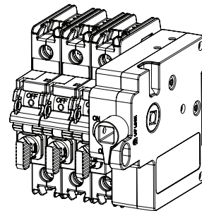
Right front rotary switch
