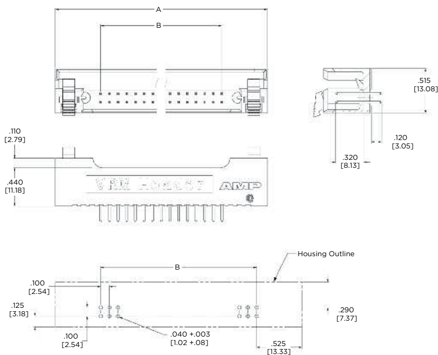
Recommended PC Board Hole Layout
