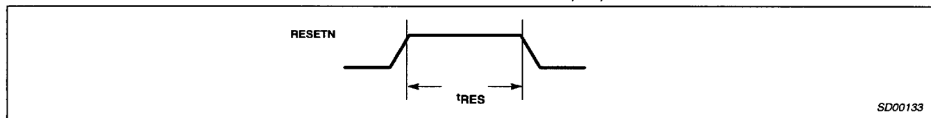
Figure 1. Reset Timing
