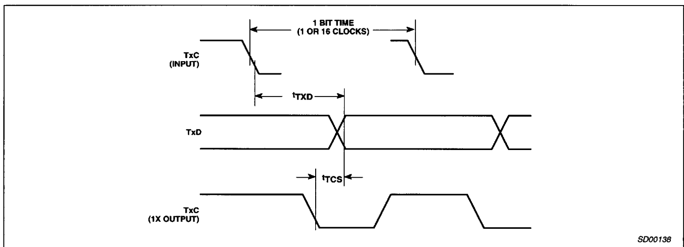
Figure 6. Transmitter External Clocks
