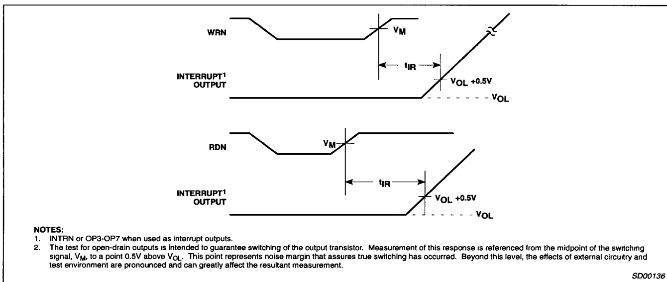
Figure 4. Interrupt Timing
