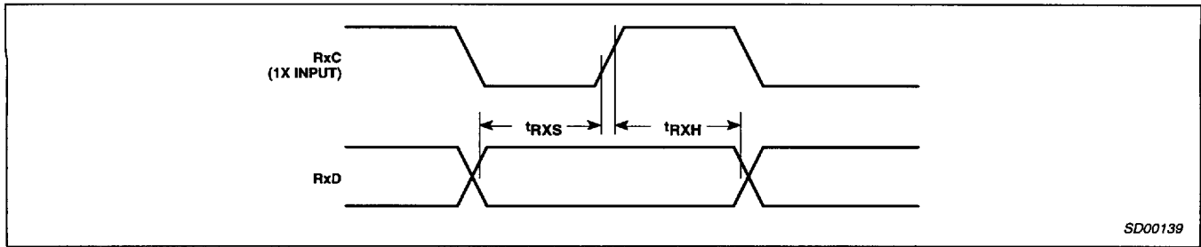
Figure 7. Receiver External Clock
