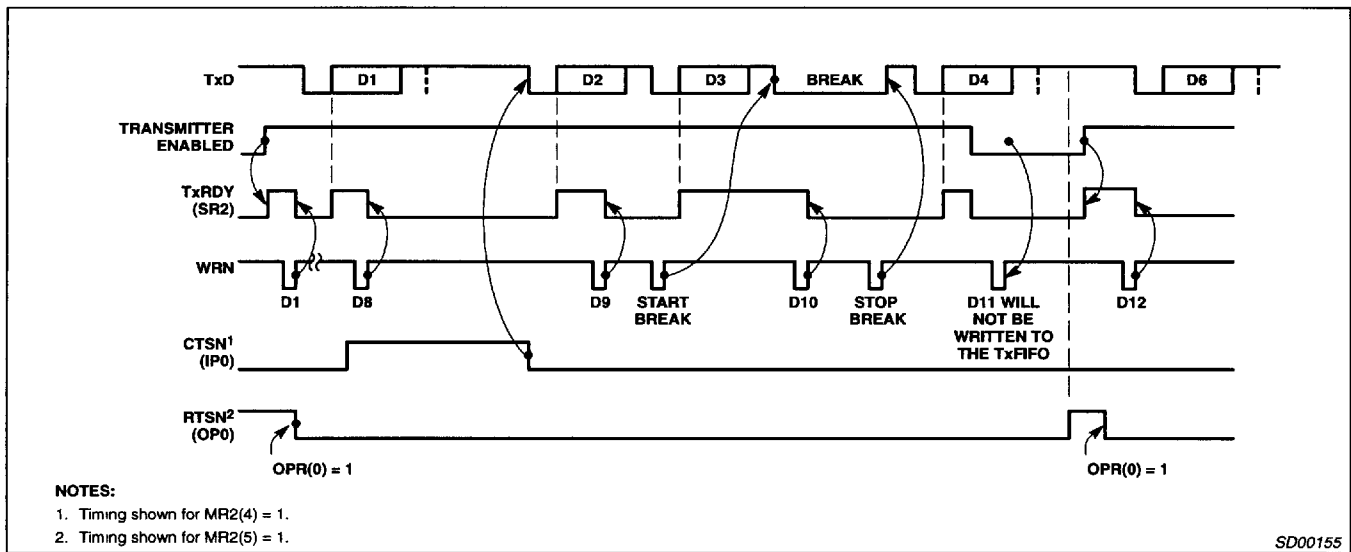
Figure 8. Transmitter Timing
