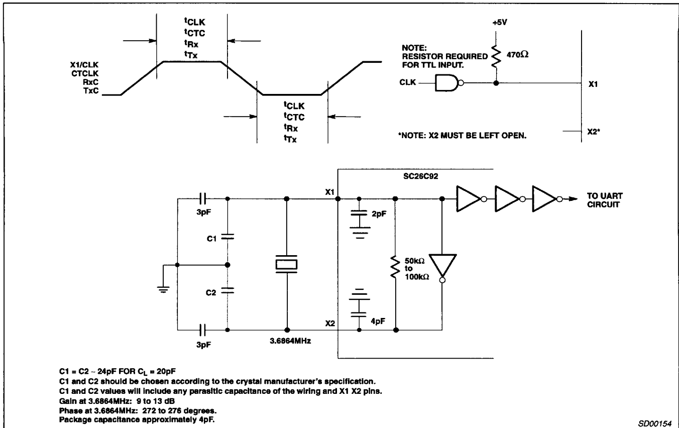
Figure 5. Clock Timing
