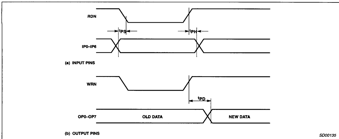
Figure 3. Port Timing
