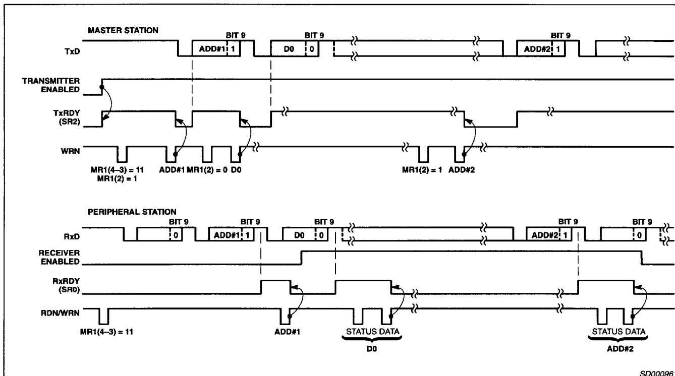
Figure 10. Wake-Up Mode
