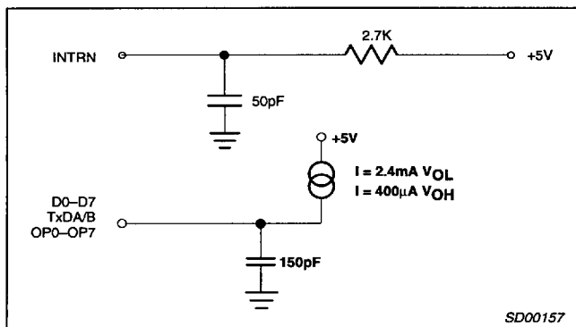
Figure 11. Test Conditions on Outputs
