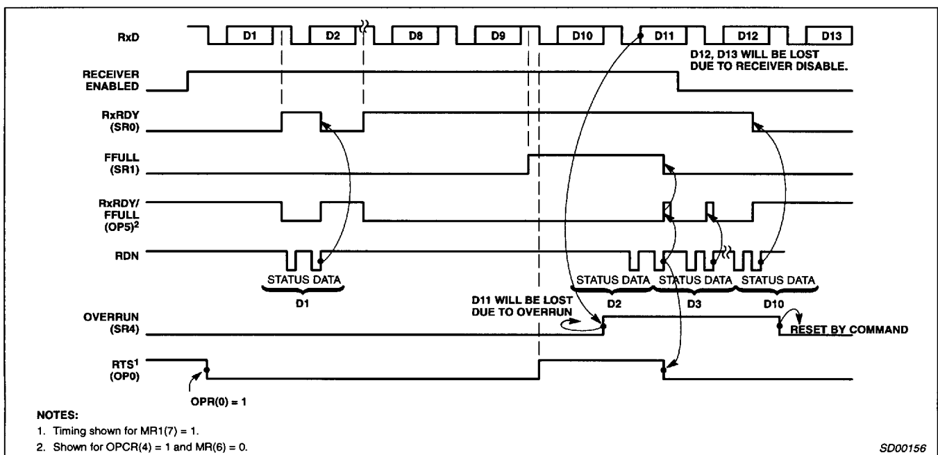
Figure 9. Receiver Timing
