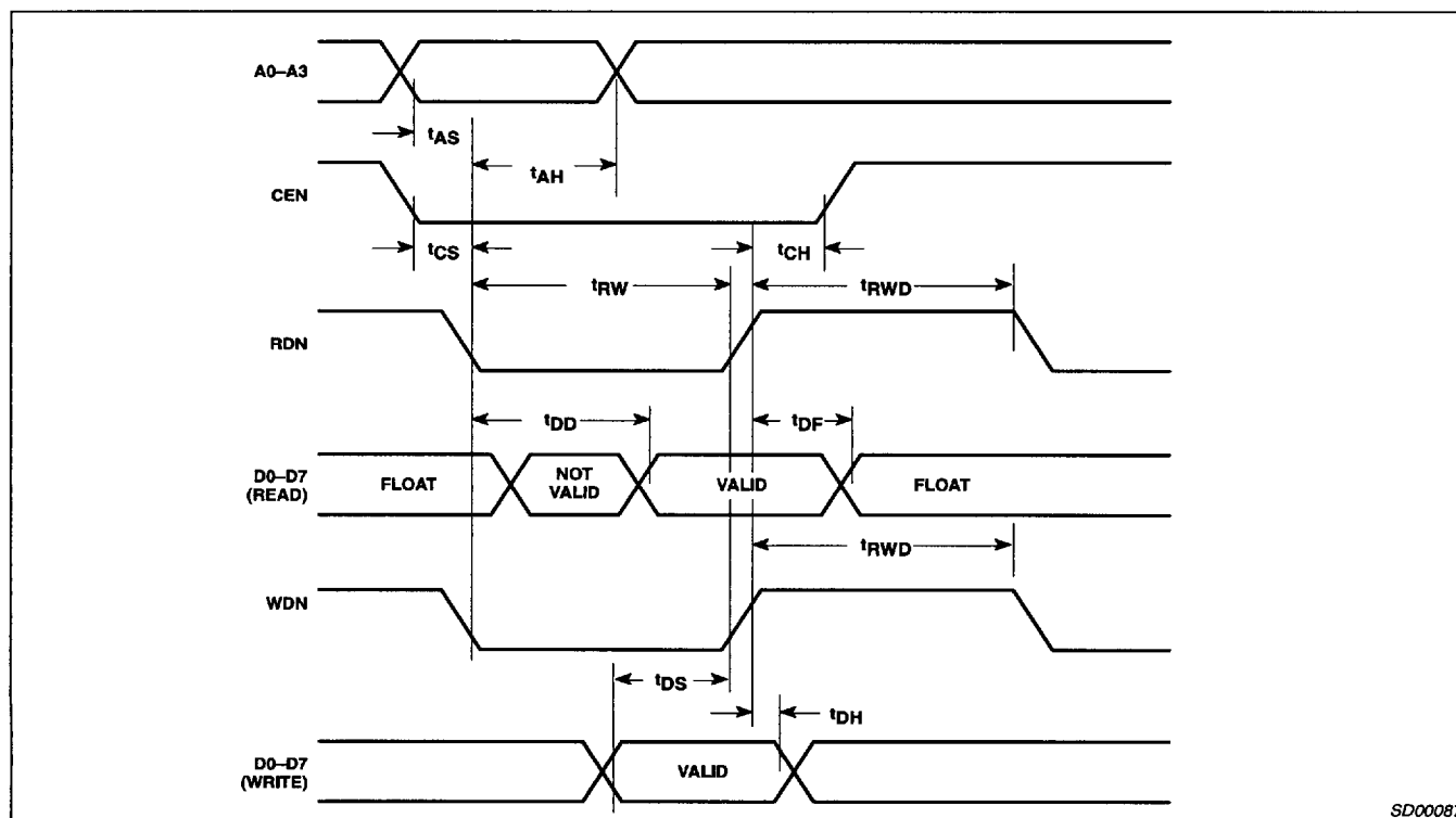
Figure 2. Bus Timing
