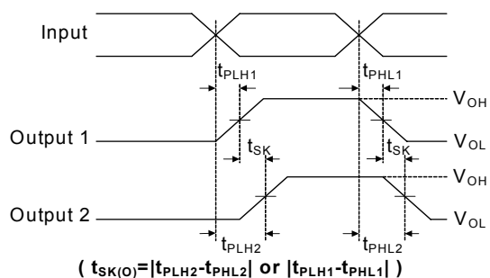
Figure 3. Output Skew
