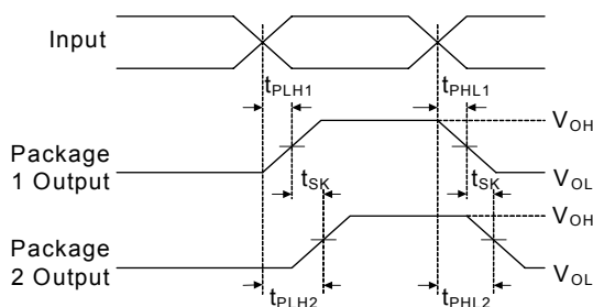
Figure 5. Part-to-Part Skew
