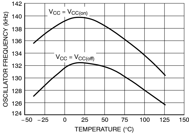
Figure 7. Oscillator Frequency (136 kHz Version) versus Temperature
