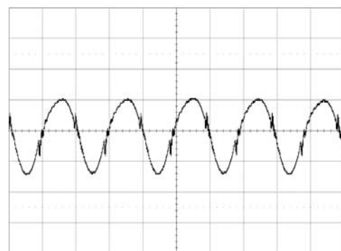
TIME, t (1 \mu s/div) Vo=5.0V, Io = Io,max
