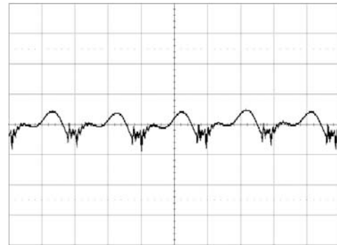
TIME, t (1 \mu s/div) Vo=1.2V, Io = Io,max
