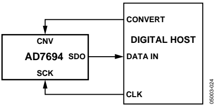
Figure 24. Connection Diagram
