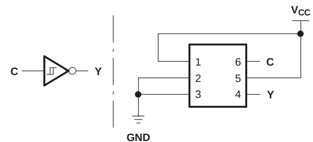
Figure 8. Inverter
