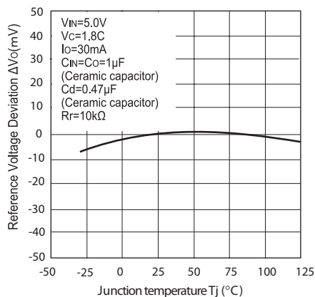
Fig.9 Reference Voltage Deviation vs. Junction Temperature (PQ1N333MASPQ)
