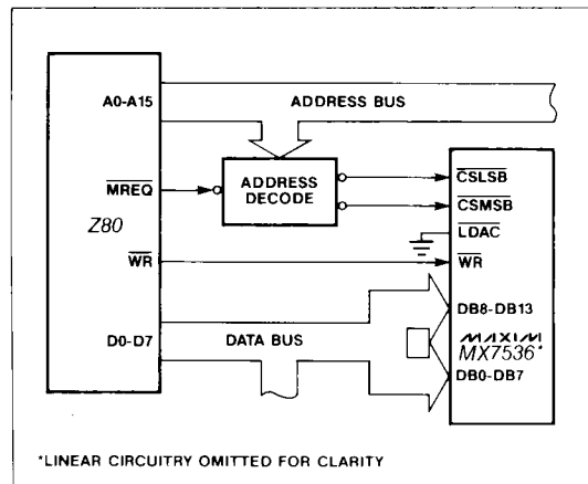
Figure 10. MX7536-Z80 Interface
