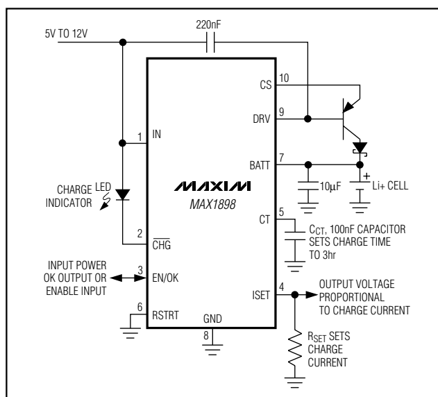
Figure 5. Application Circuit with PNP Pass Transistor
