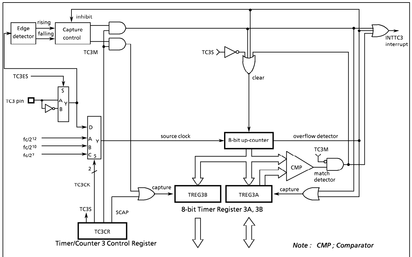
Figure 2-21. Timer/Counter (TC3)
