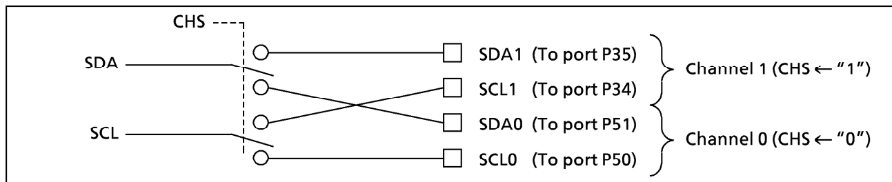
Figure 2-31. Channel Selection
