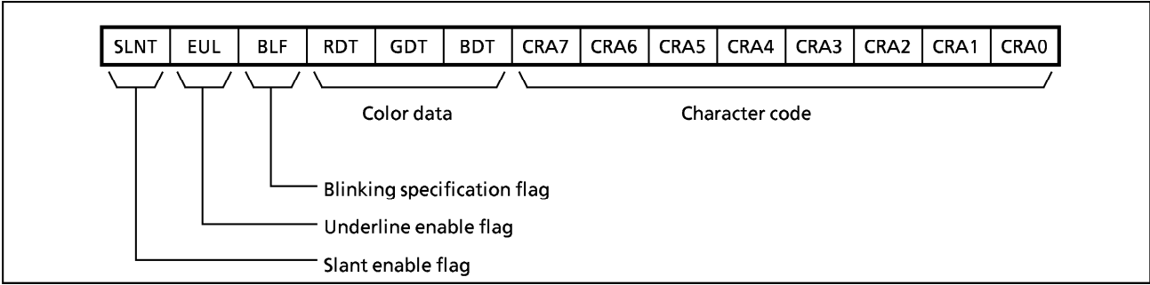
Figure 2-66. Display Memory Bit Configuration
