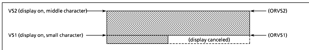
Figure 2-72. Occasion of Overlapping ( VS1 > VS2 )
