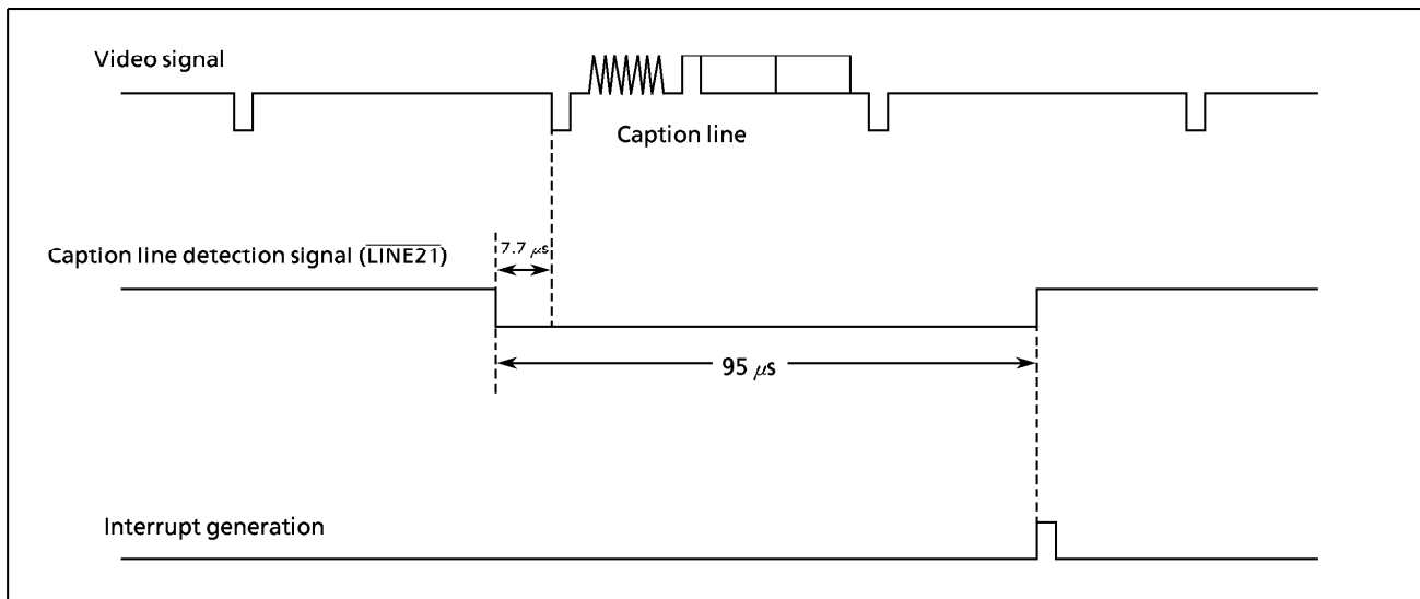
Figure 2-90. Interrupt Generation Timing
