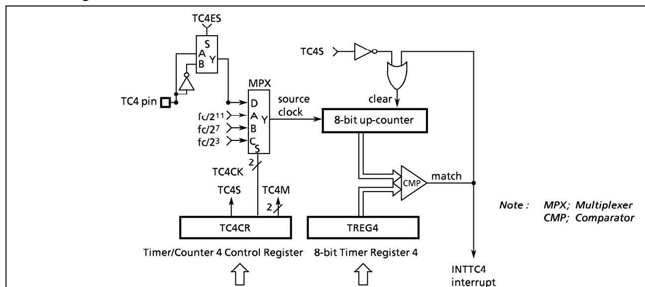
Figure 2-24. Timer/Counter 4
