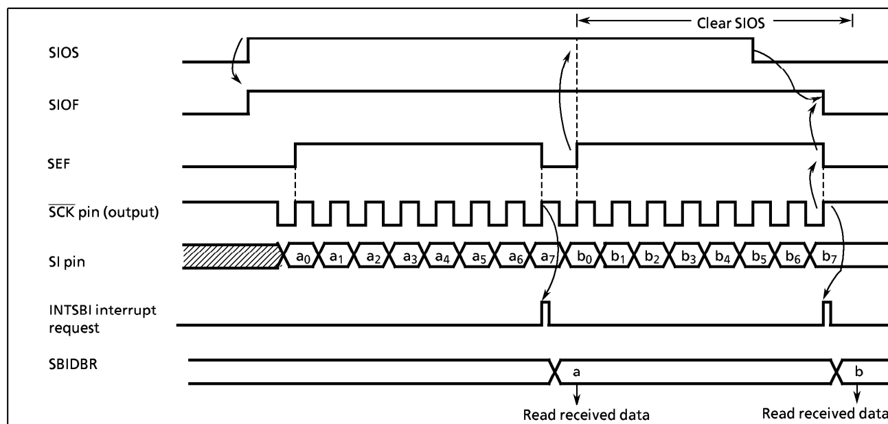
Figure 2-47. Receive Mode (Example : Internal clock)
