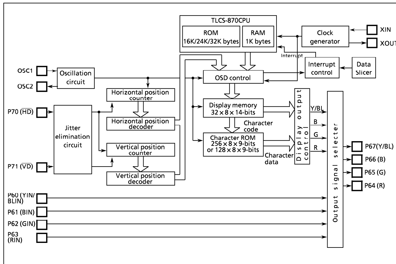
Figure 2-64. OSD Circuit
