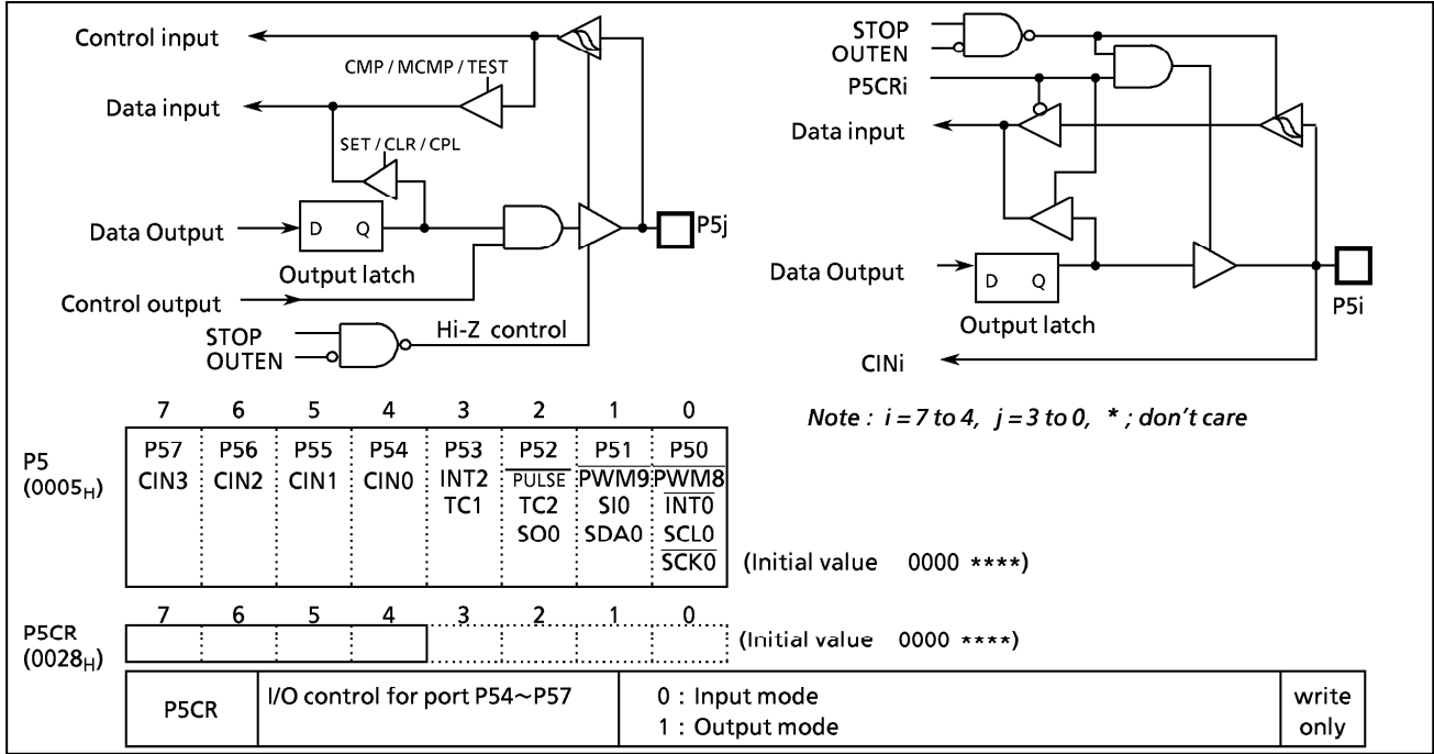
Figure 2-6. Ports P5
