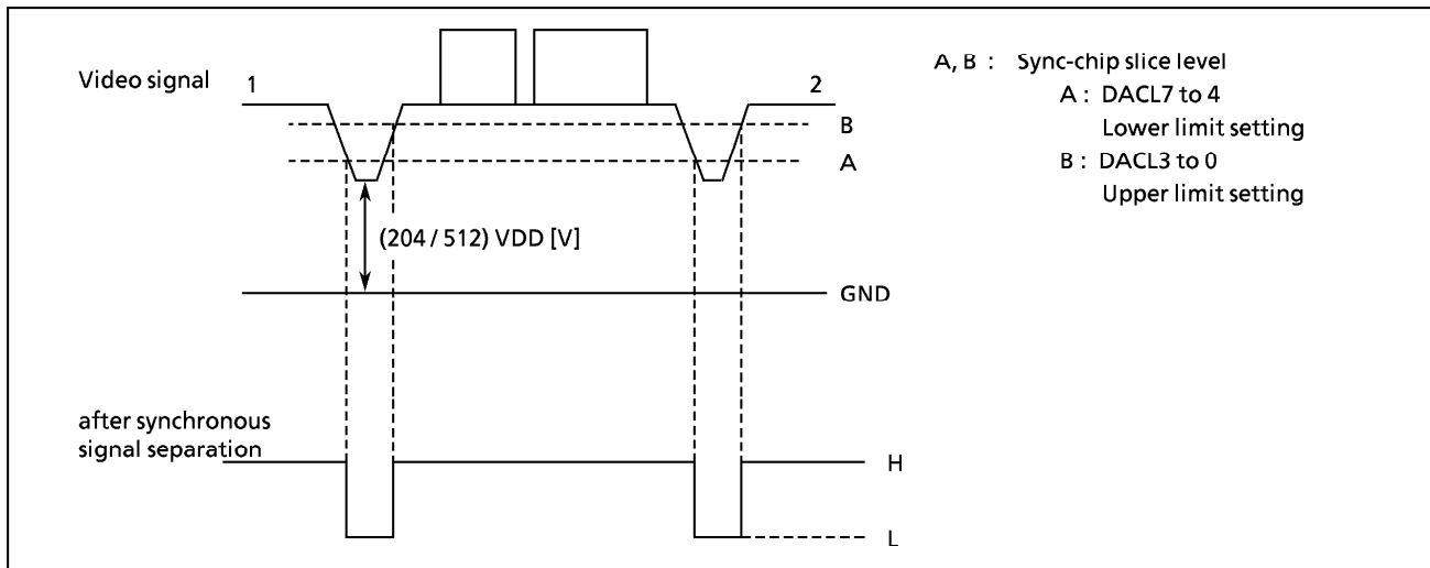
Figure 2-93. Synchronous Signal Slice
