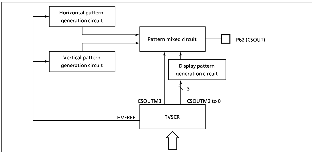
Figure 2-95. TEST Video Signal Output Circuit
