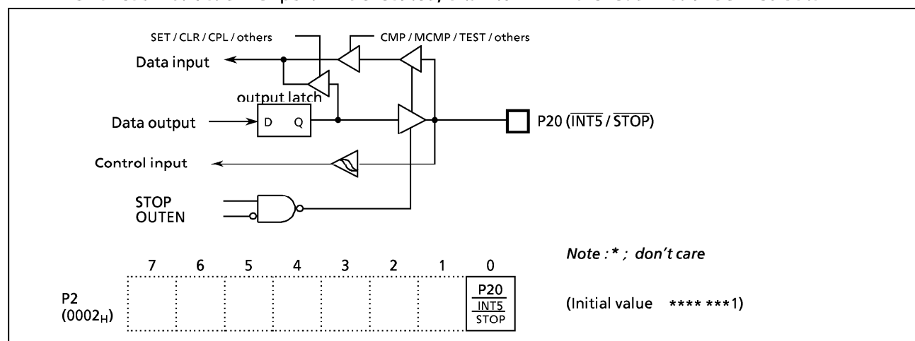
Figure 2-3 Port P2
