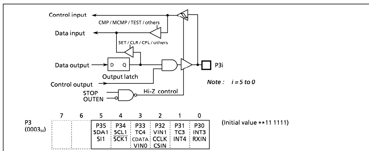
Figure 2-4 Port P3
