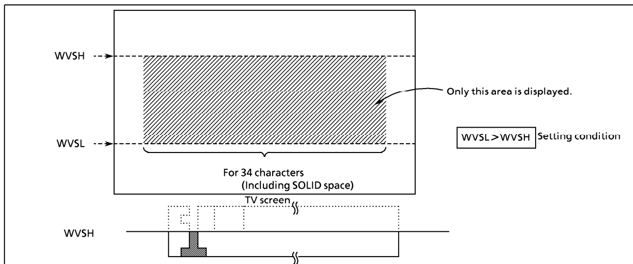
Figure 2-80. Window
