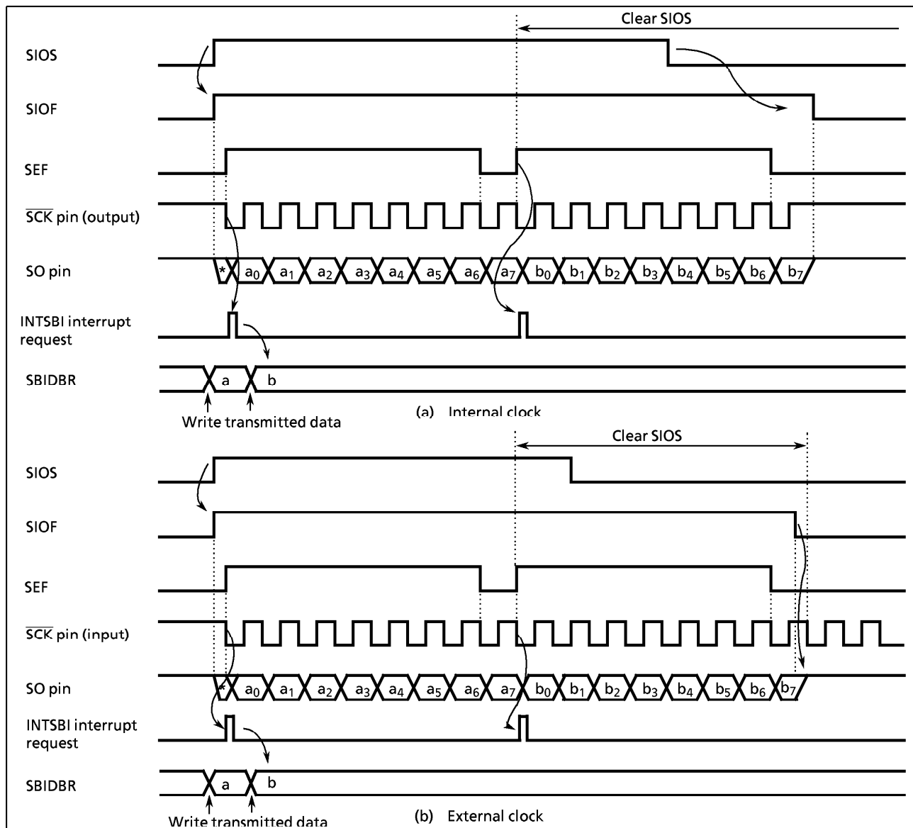
Figure 2-45. Transfer Mode
