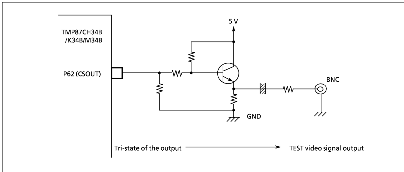
Figure 2-98. Example of Test Video Output Generation
