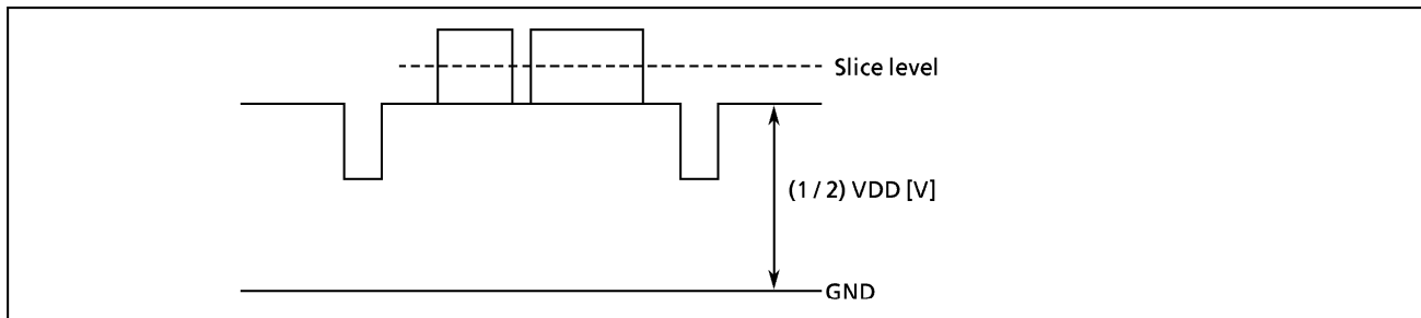
Figure 2-94. Pedestal Clamp
