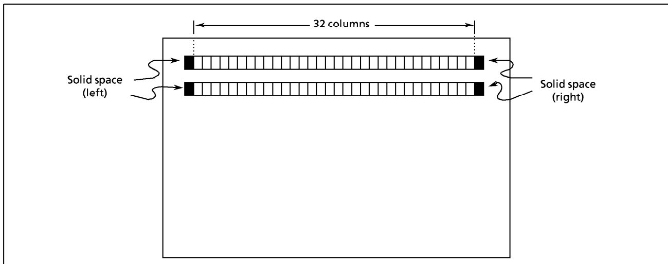
Figure 2-78. Solid Space
