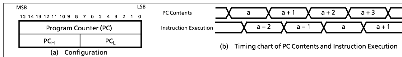
Figure 1-3. Program Counter
