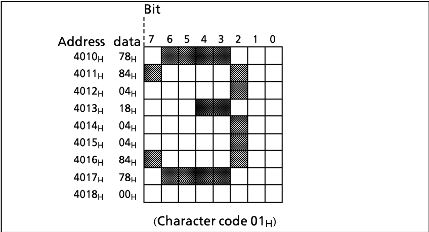
Figure 2-65. 8 × 9 Dot Pattern Configuration
