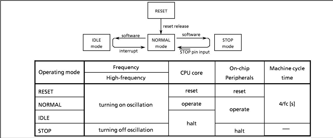
Figure 1-13. Operating Mode Transition Diagram
