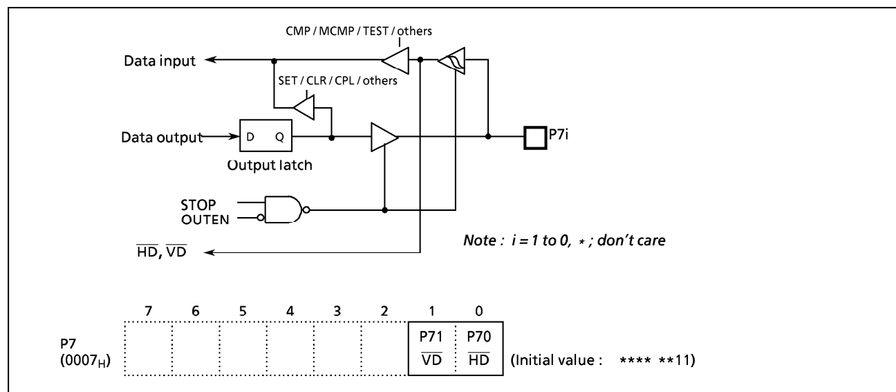
Figure 2-8. Ports P7
