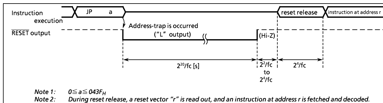
Figure 1-29. Address-Trap-Reset
