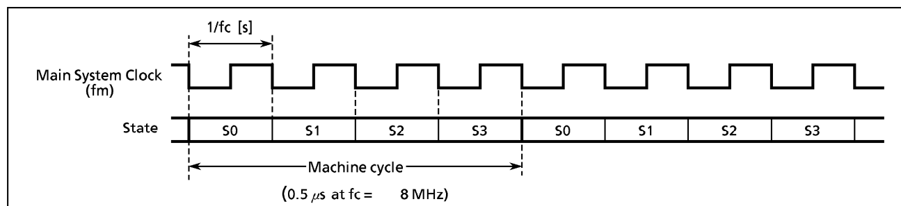
Figure 1-12. Machine Cycle
