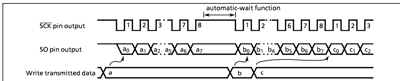
Figure 2-42. Automatic-wait Function
