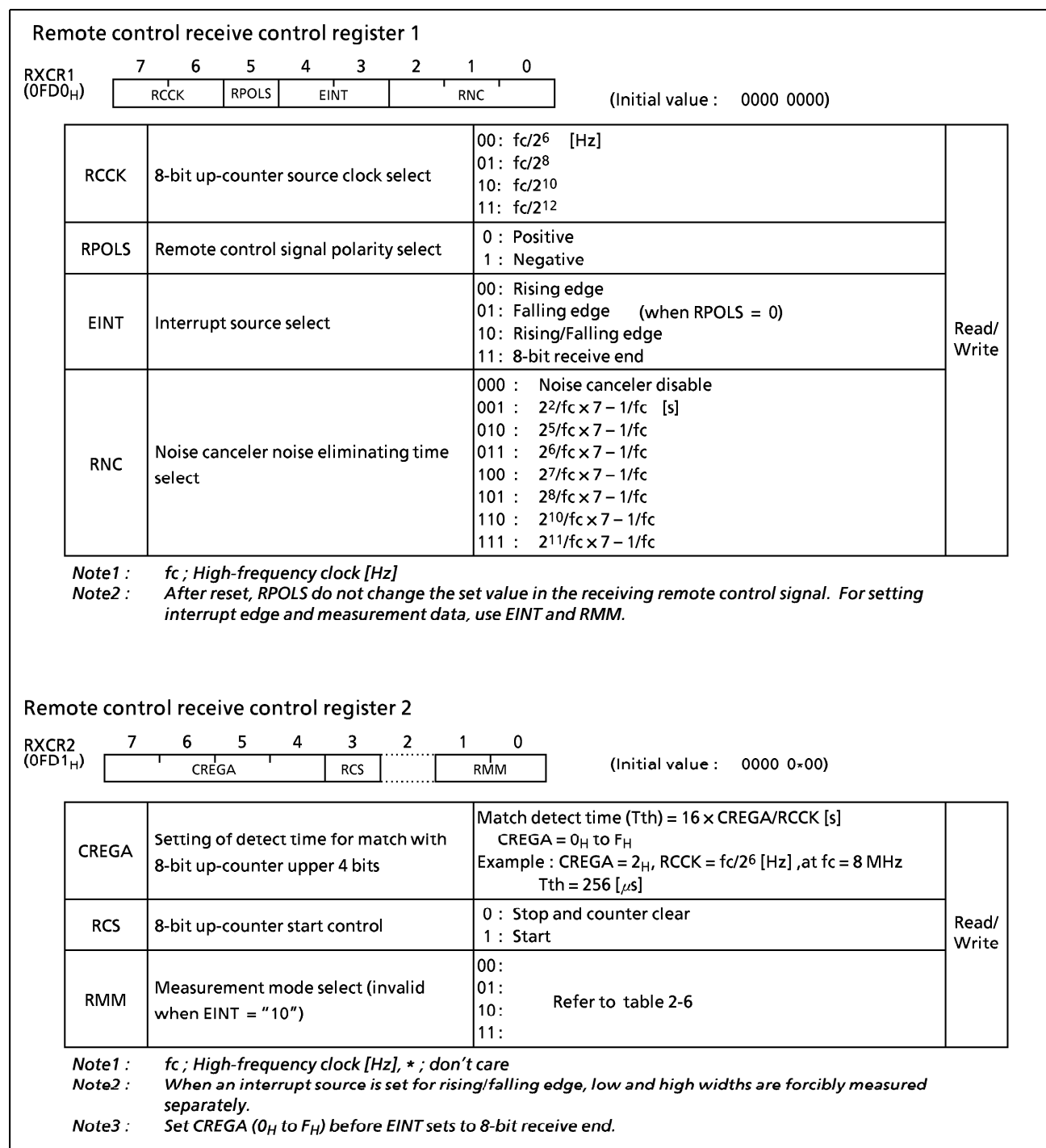
Figure 2-51. Remote Control Receive Control Register 1, 2
