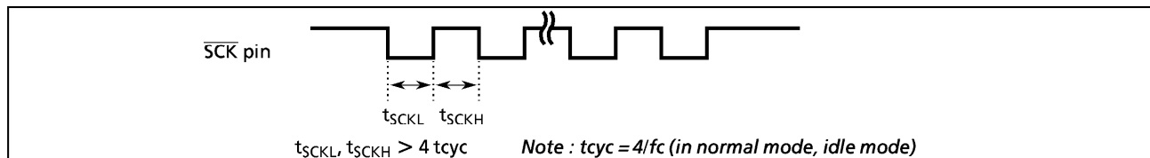
Figure 2-43. External Clock
