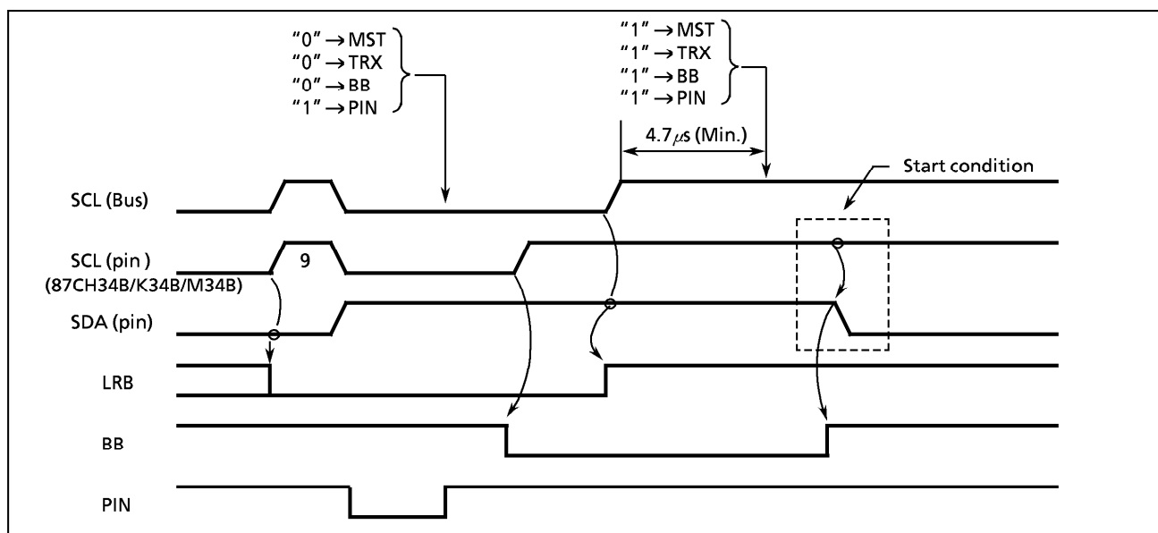
Figure 2-40. Timing Diagram when Restarting the 87CH34B/K34B/M34B
