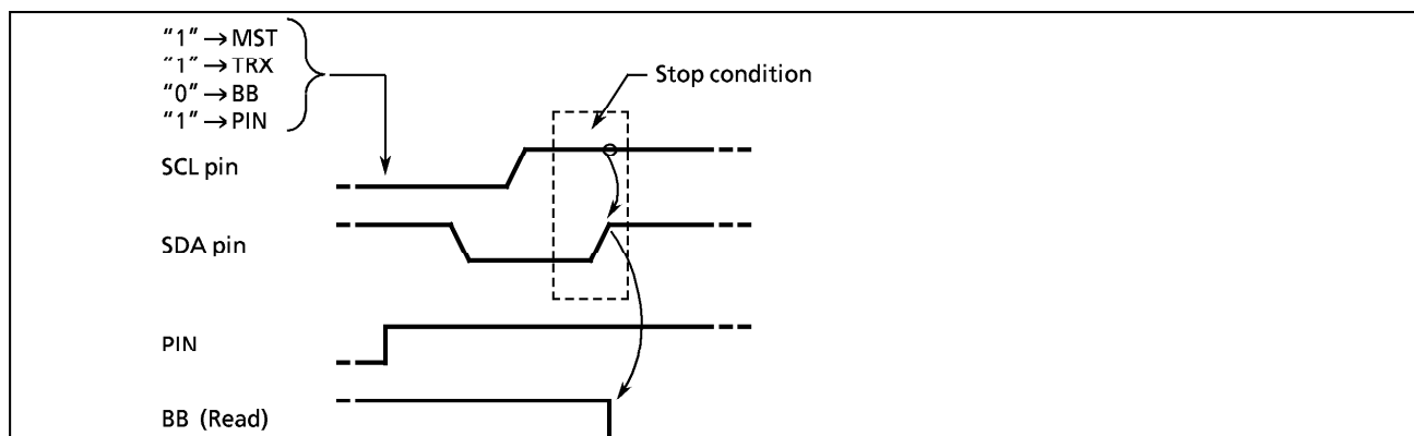
Figure 2-39. Stop Condition Generation
