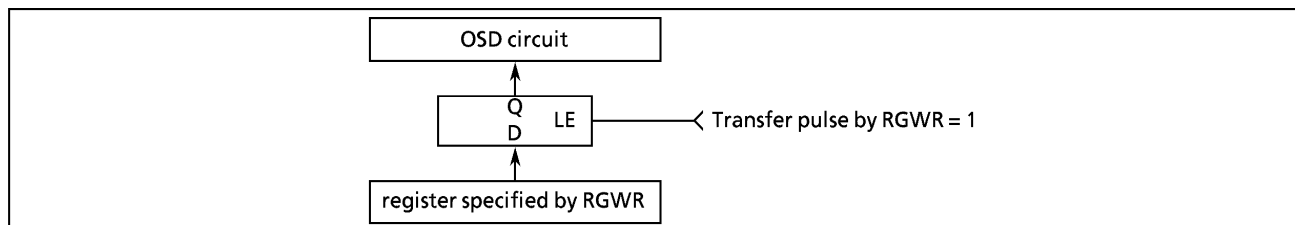
Figure 2-82. RGWR System
