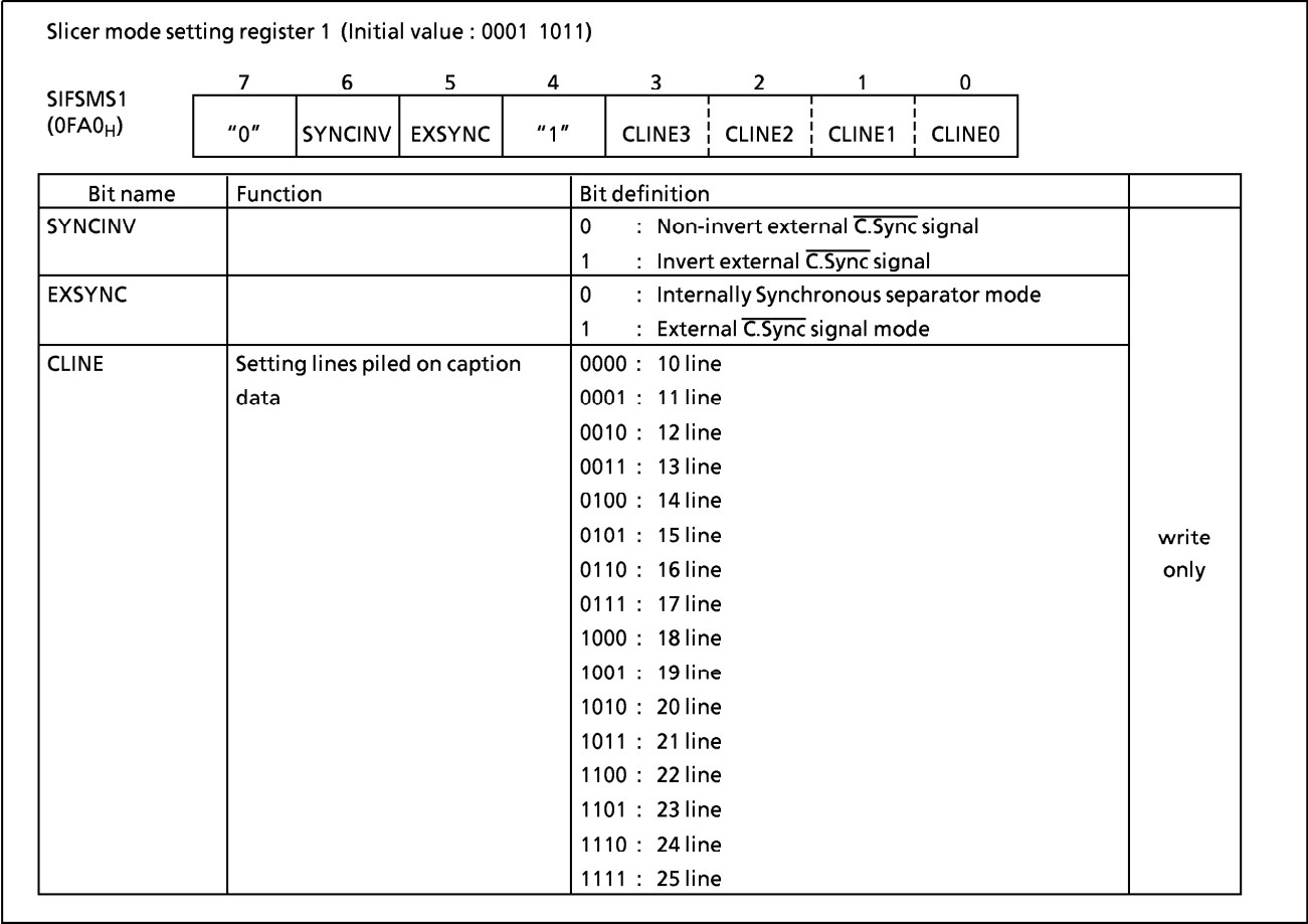
Figure 2-92-3. Slicer Mode Setting Register
