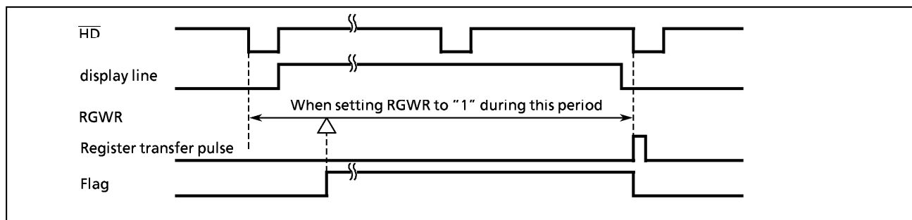
Figure 2-84. Data Transfer Timing in Display Area
