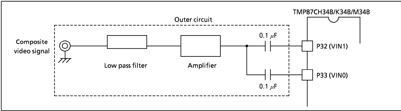
Figure 2-91. Video Signal Connection
