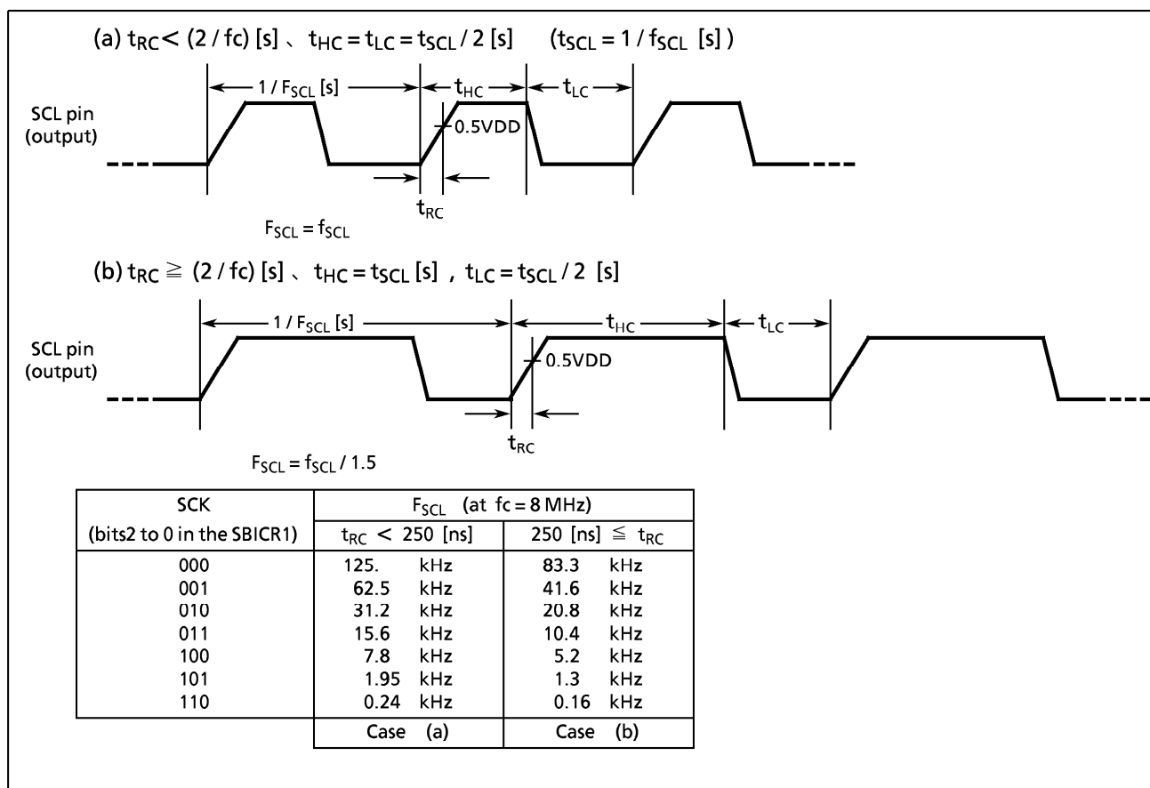
Figure 2-32. Serial Clock
