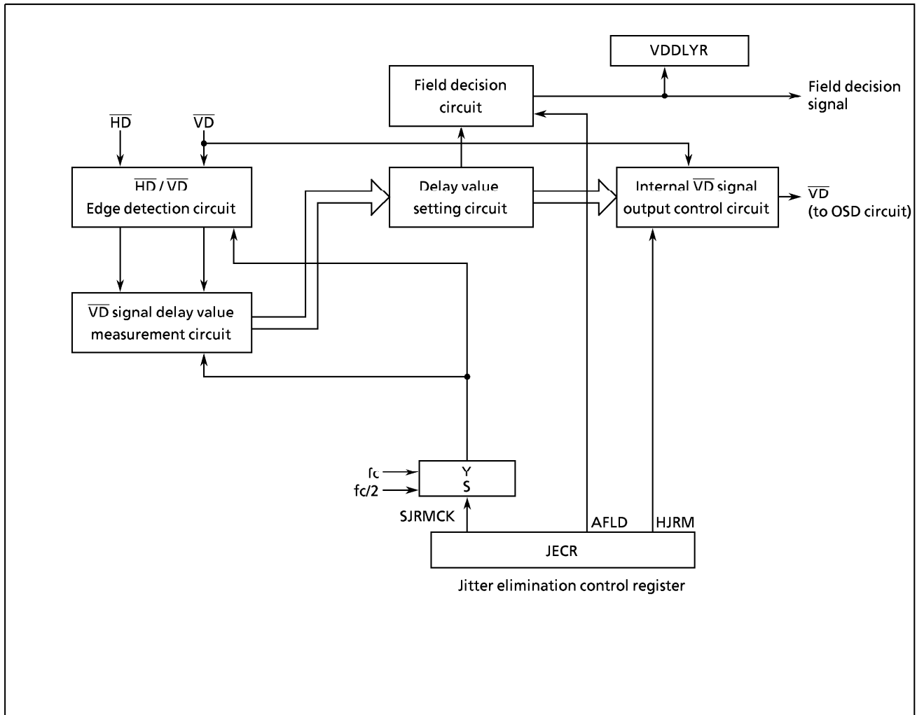
Figure 2-85. Jitter Elimination Circuit
