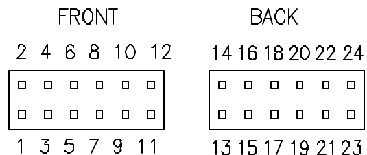
24 LEAD SSOP PIN LAYOUT
