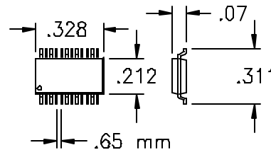
24 PIN SSOP CHIP
