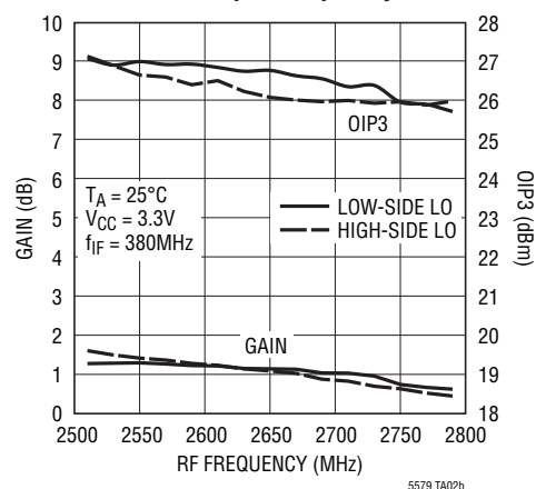
Gain and OIP3 vs RF Output Frequency
