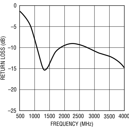
Figure 5. LO Input Return Loss
