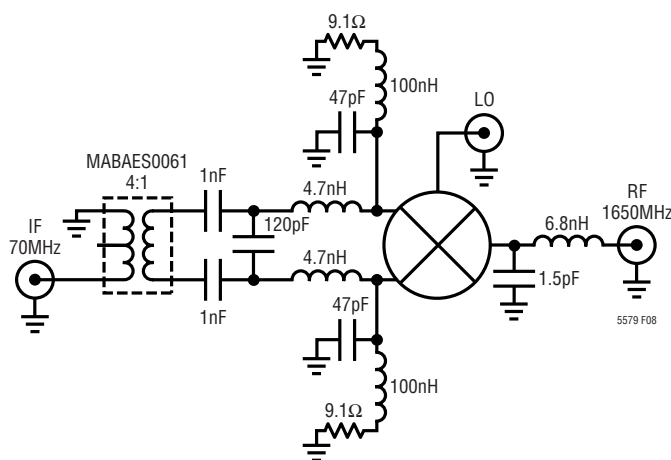
Figure 8. IF Input Tuned for 70MHz
