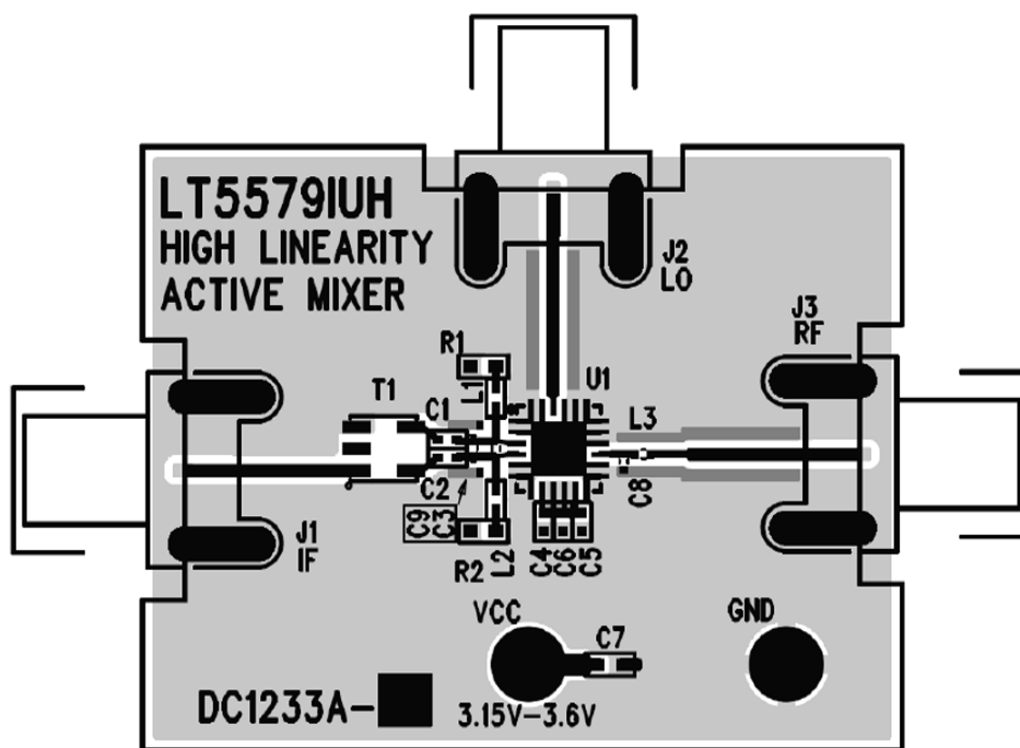
Figure 12. LT5579 Evaluation Board (DC1233A)
