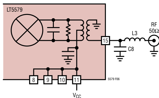
Figure 6. RF Output Circuit
