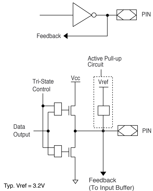
Typical Output
