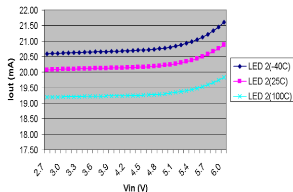
Fig. 10: Line Regulation LED1 DAC = 101000 (20mA)
