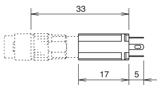
Solder Terminal (AL-C8)
