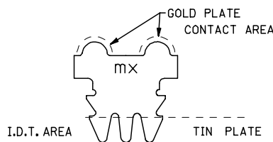
SIDE VIEW OF CONTACT
