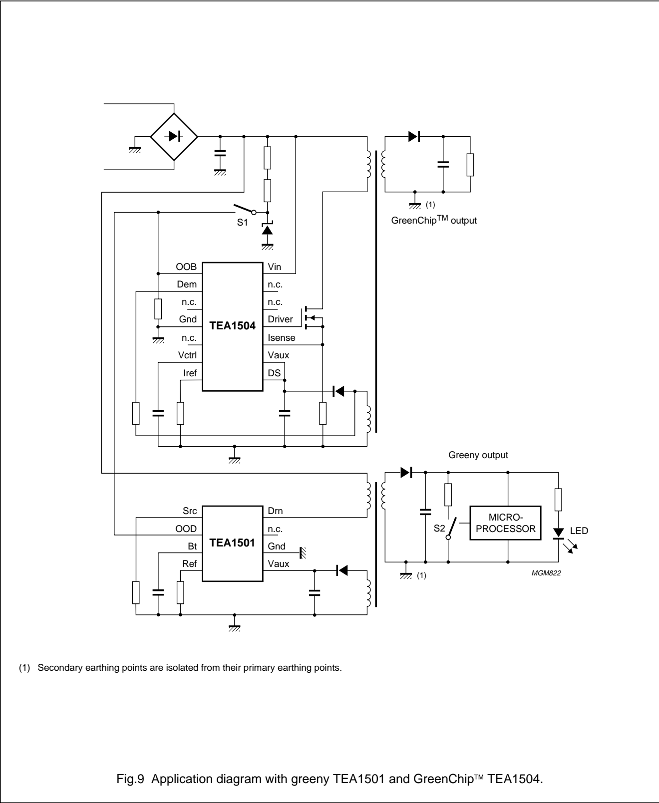
APPLICATION DIAGRAM WITH GREENY TEA1501 AND GREENCHIP™ TEA1504
