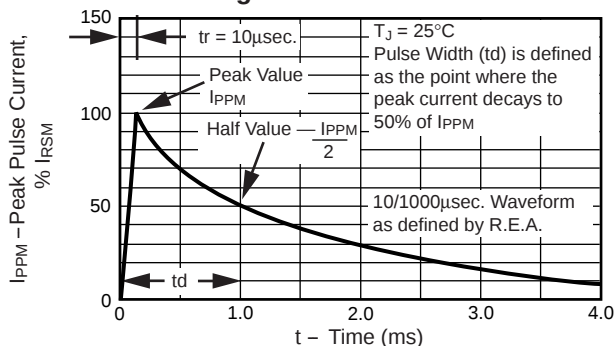
Fig. 3 – Pulse Waveform
