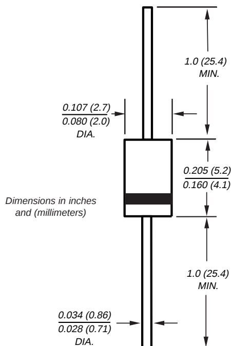
DO-204AL (DO-41 Plastic)
