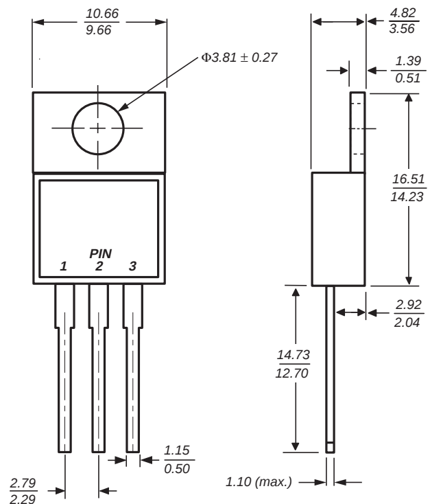
TO-220 Case Outline
