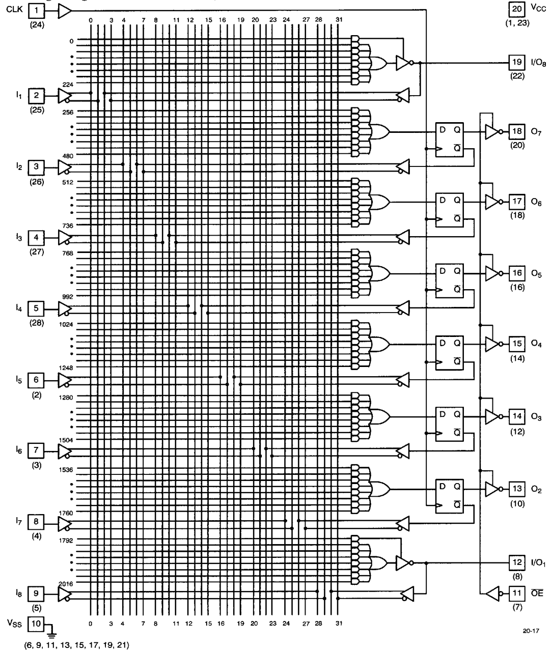
16R6 Logic Diagram 20-Pin DIP/PLCC/LCC (28-Pin PLCC) Pinouts
