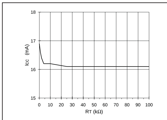
I CC vs R_T with Opposite R_T = 50k
