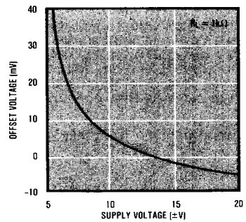
OFFSET VOLTAGE vs SUPPLY VOLTAGE
