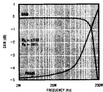
FREQUENCY RESPONSE
