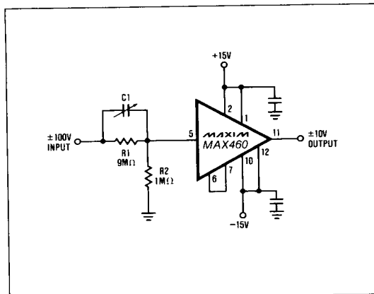
Figure 5. High Speed High Voltage Attenuator
