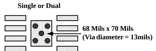
Figure 112. PowerPAD PCB Etch and Via Pattern
