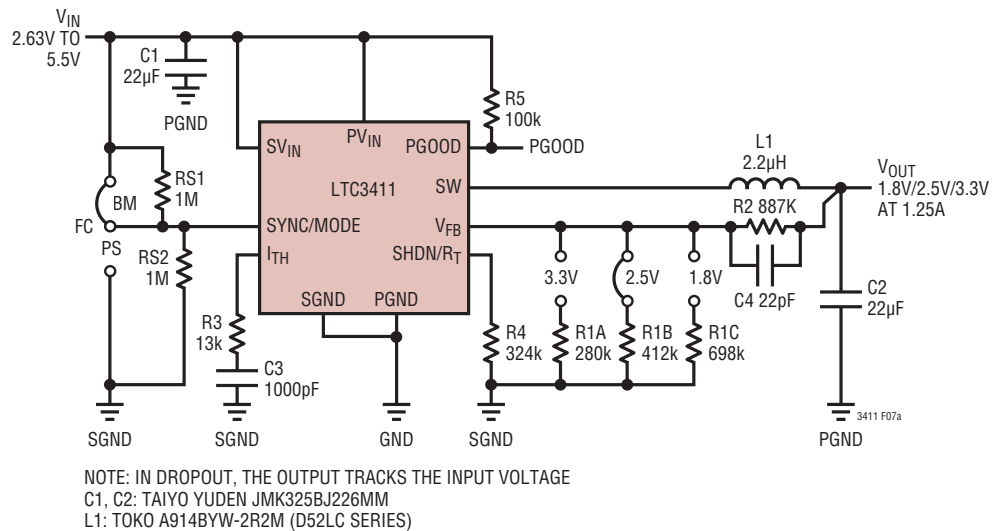
Figure 7. General Purpose Buck Regulator Using Ceramic Capacitors
