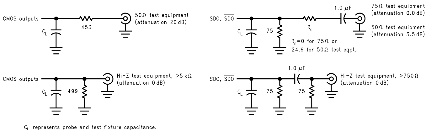
Figure 2. Test Loads
