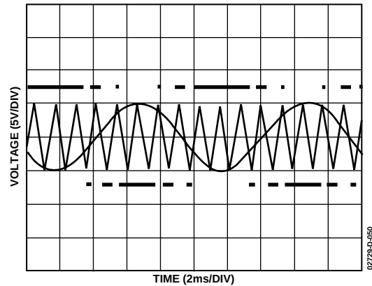
Figure 56. Pulse-Width Modulation
