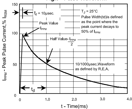
Fig.3 - Pulse Waveform
