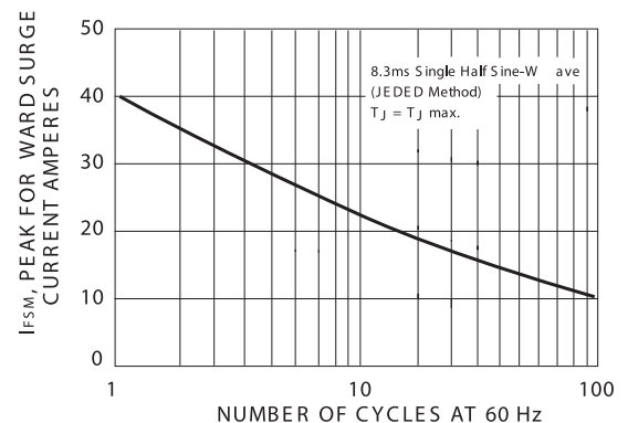
FIG. 4 - MAXIMUM NON-REPETITIVE FORWARD SURGE CURRENT UNIDIRECTIONAL
