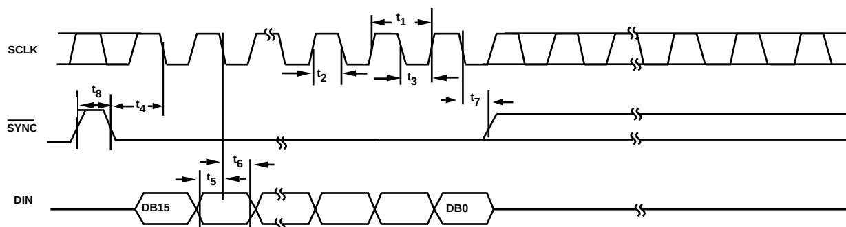
Figure 1. Timing Diagram.
