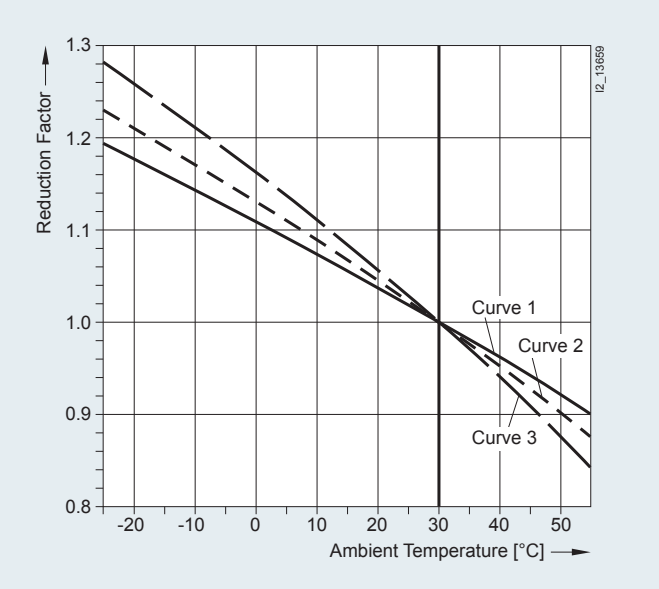
Curve for correction factor (for curves, see the diagram above)
