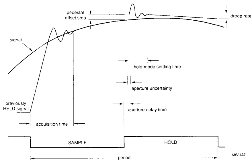
Fig.4 Sample/hold timing characteristics (not to scale).
