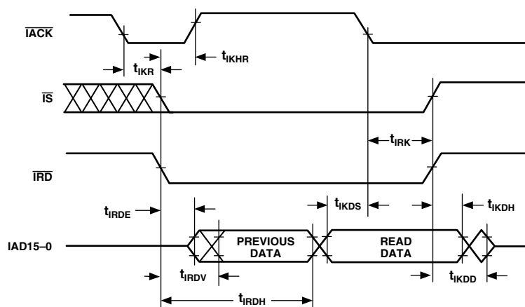
Figure 24. IDMA Read, Long Read Cycle
