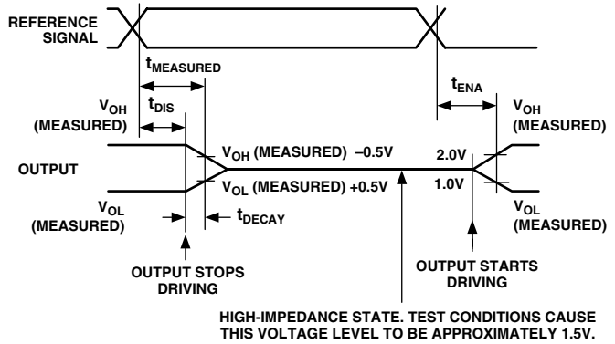
Figure 16. Output Enable/Disable
