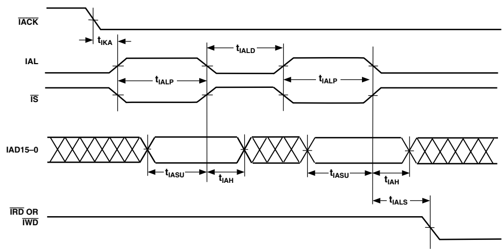
Figure 21. IDMA Address Latch
