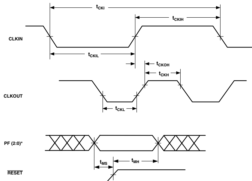
Figure 18. Clock Signals
