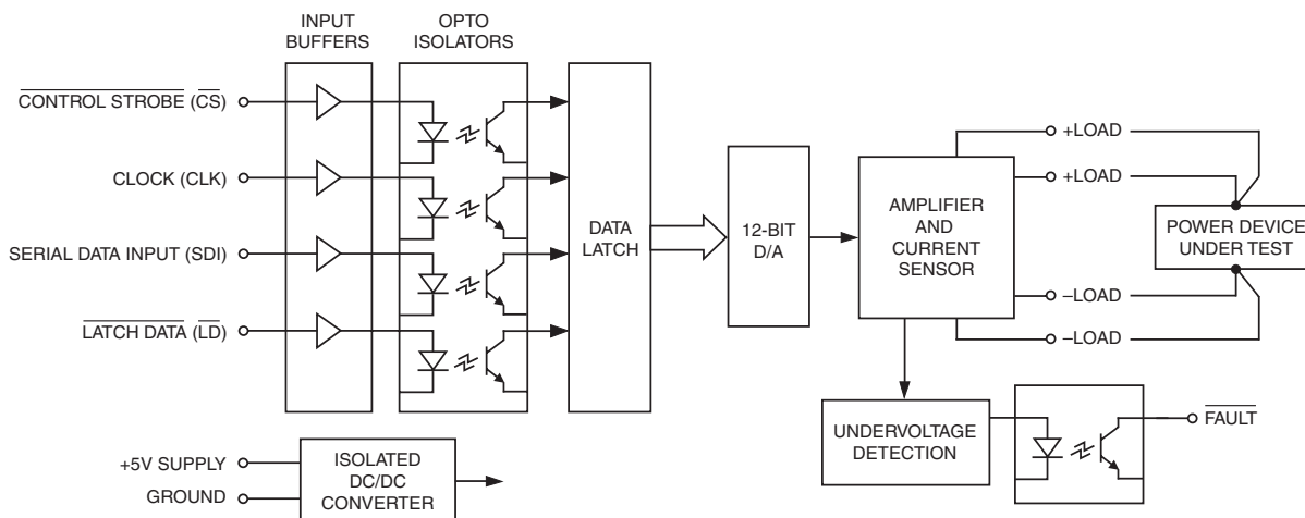
Figure 1. Simplified Schematic
