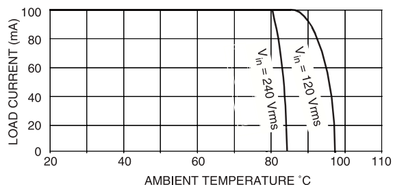
LOAD CURRENT VS AMBIENT TEMPERATURE FIGURE 3
