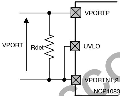
Figure 11. Default UVLO Settings
